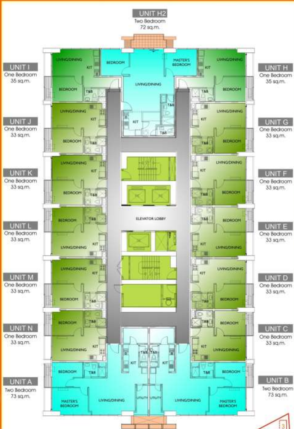
9th to 35th Odd Numbered Floor Plan
